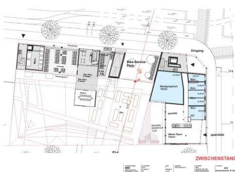
EG-Grundriss C.22.B © AG3
